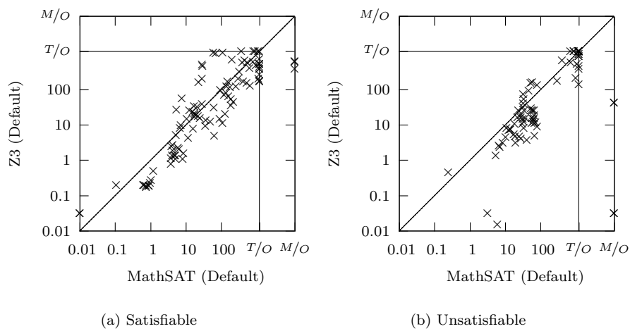
Fig. 7: Comparison of bit-blasting-based decision procedures.
