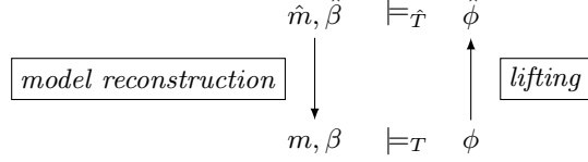
Fig. 1: Commutativity graph showing how the model m, \beta can be obtained via approximation theory \hat{T} .
