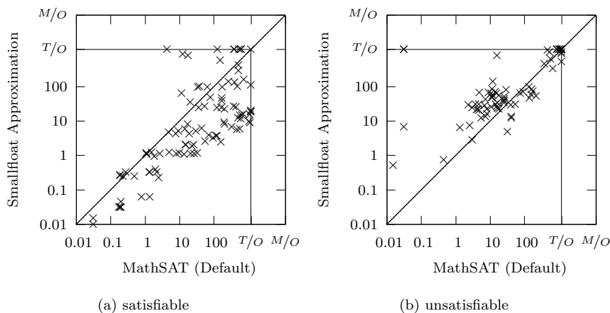
Fig. 4: Comparison of our approximation method with the bit-blasting-based decision procedure in MathSAT.
