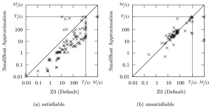
Fig. 3: Comparisons of our method with the bit-blasting-based decision procedure in Z3.
