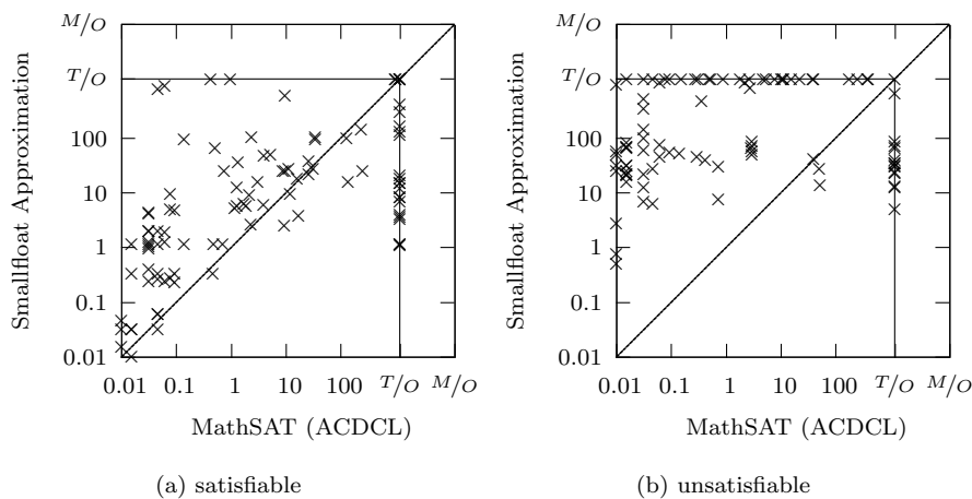
Fig. 5: Comparison of our approximation method with the ACDCL-based decision procedure in MathSAT.
