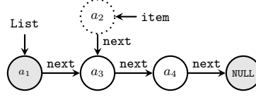
Figure 2. A possible heap resulting from three inserts and one pop .
