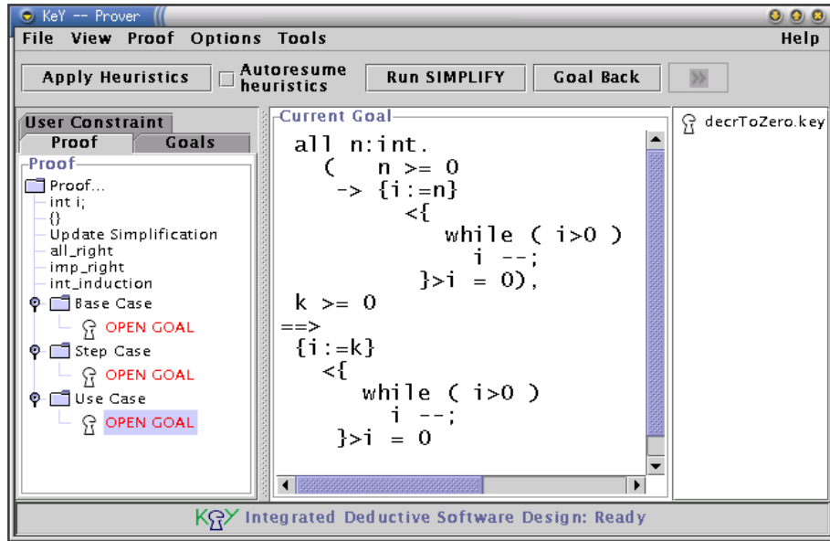
Figure 2. Annotated Proof Tree after Applying Tactlet for Induction
